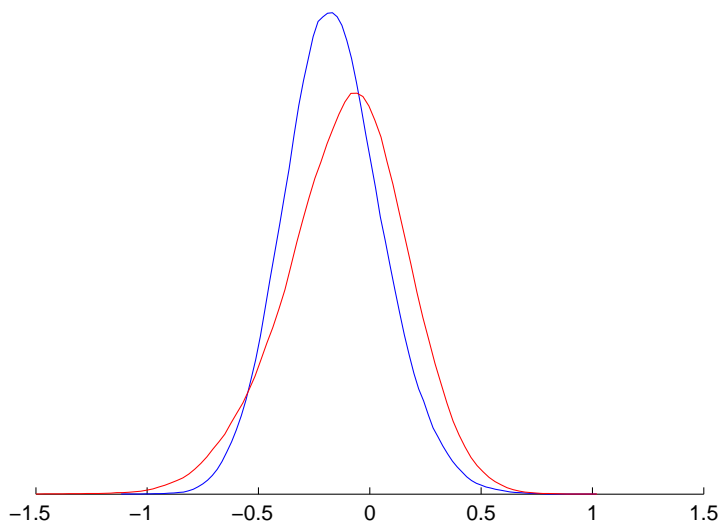
Figure 9.4: Estimate of the posterior distribution for \theta_{S1} , the effect of length on the logit of survival before the regulation (blue line) and \theta_{S4} , the effect of age on the logit of survival (red line).
