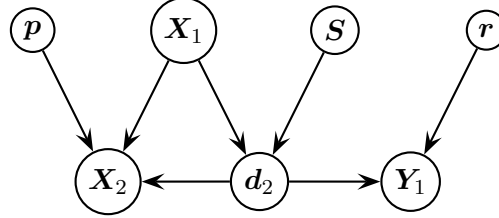
Figure 4.5: A DAG for the CJS model with auxiliary data on dead recoveries. This is the dead recovery model of Burnham (1993) with no movement.
