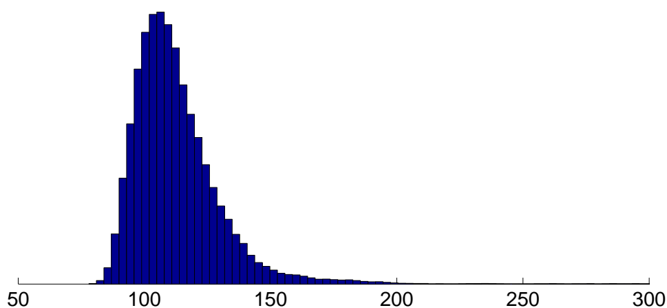
Figure 7.2: Posterior density estimate for the population size \aleph for model M_h with individual-specific covariates that are assumed to be drawn from a common normal distribution. The data were simulated with a true population size of 100.
