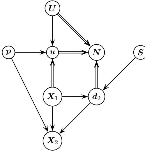
Figure 3.5: A DAG for the JS model including the population size in each sample \mathbf{N} = (N_1, \dots, N_k) .
