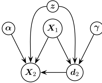
Figure 4.2: A DAG for the CJS model where the covariate \mathbf{z} fully explains capture and survival probability.
