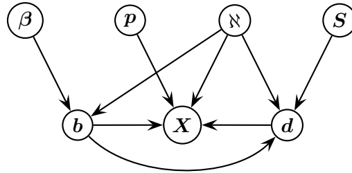
Figure 3.6: A DAG for the CMAS model.
