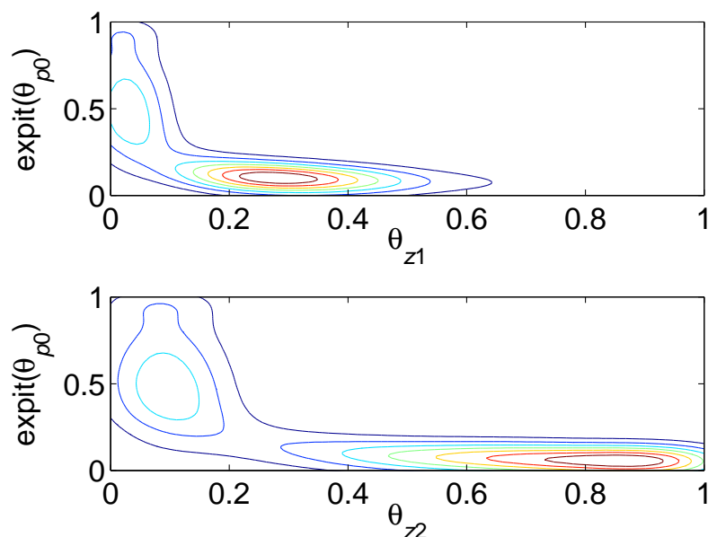
Figure 9.8: Contour plot of the estimate of the joint posterior distribution for the parameters \theta_{z1} and \text{expit}(\theta_{p0}) (top) and \theta_{z2} and \text{expit}(\theta_{p0}) (bottom).
